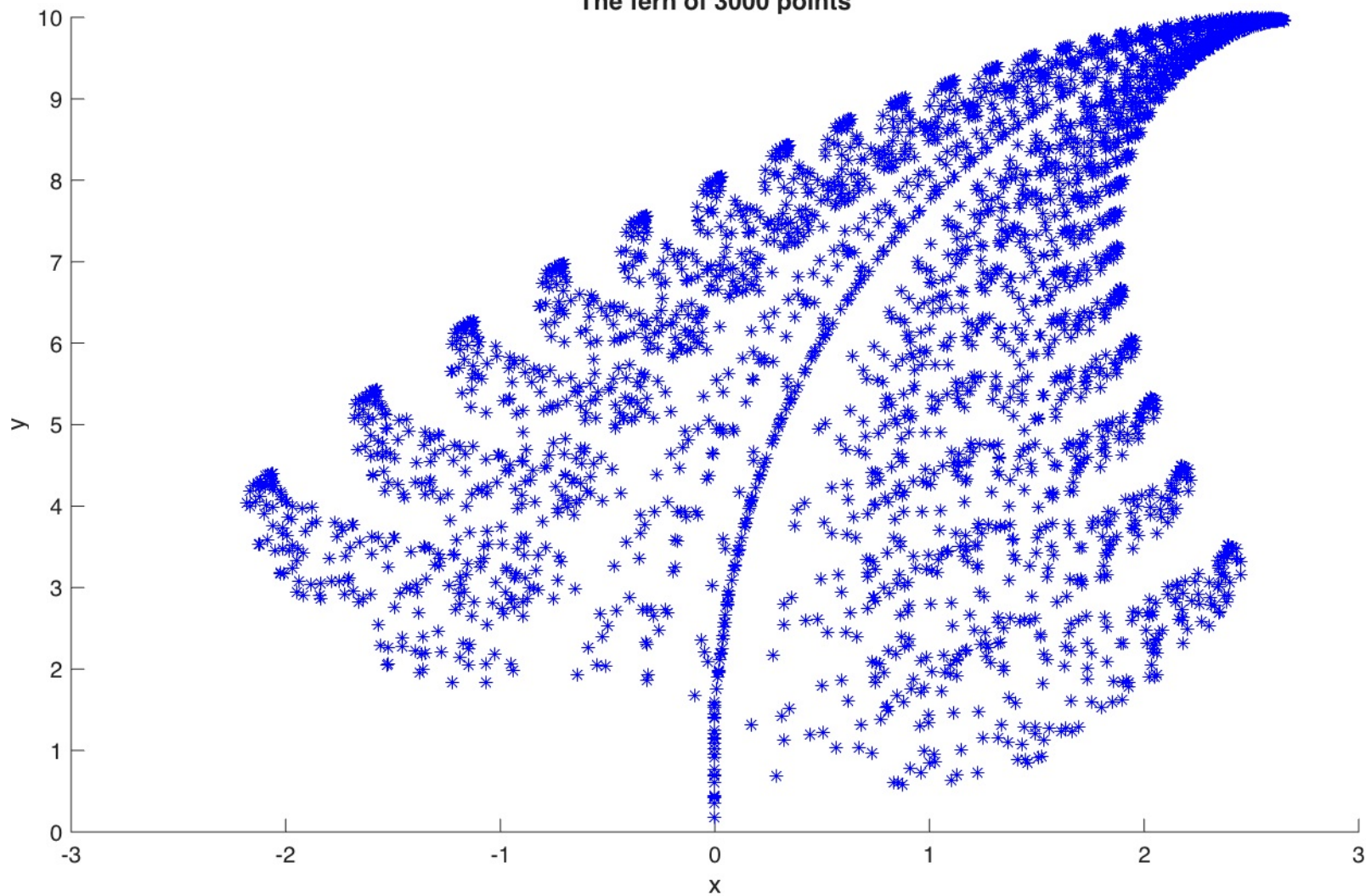
The fern of 3000 points
